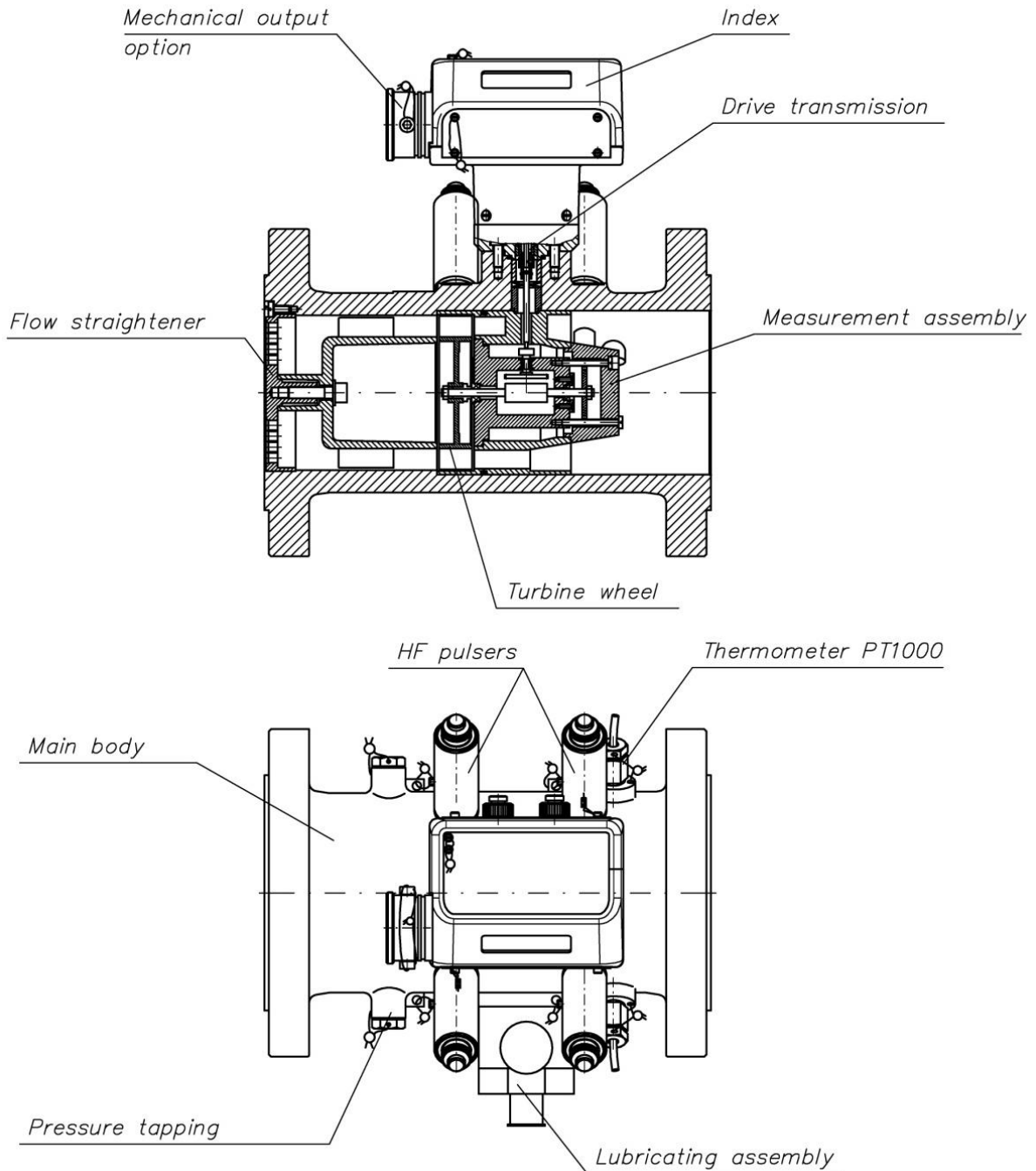
Fig. 2 Cross-section of the turbine gas meter CGT-02
